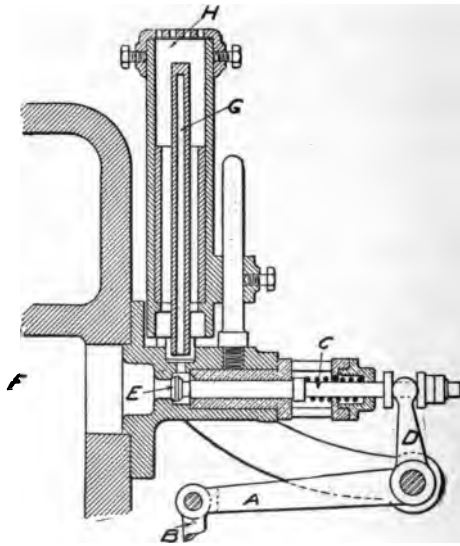
FIG. 169.—A Hot Tube Igniter, with a Geared Timing Attachment for Regulating the Point of Firing. G is the hot tube enclosed with a cylindrical case having a perforated cap, H, at the top. The heat of the tube is maintained by a gas flame within the cylindrical case. The link, B, operates the levers, A and D, so as to open the valve, E, which is normally held closed by the spring, C, bearing on its rod as shown. In opening the valve to the point in the cycle at which the cam actuates the link, B, thus compressing the spring, C, and opening the valve, D, the interior of the hot tube, G, is brought into communication with the combustion chamber, F, of the cylinder. The time of ignition may be varied by adjusting the throw of the cam, so as to bring the opening of the valve, E, to any desired point.
